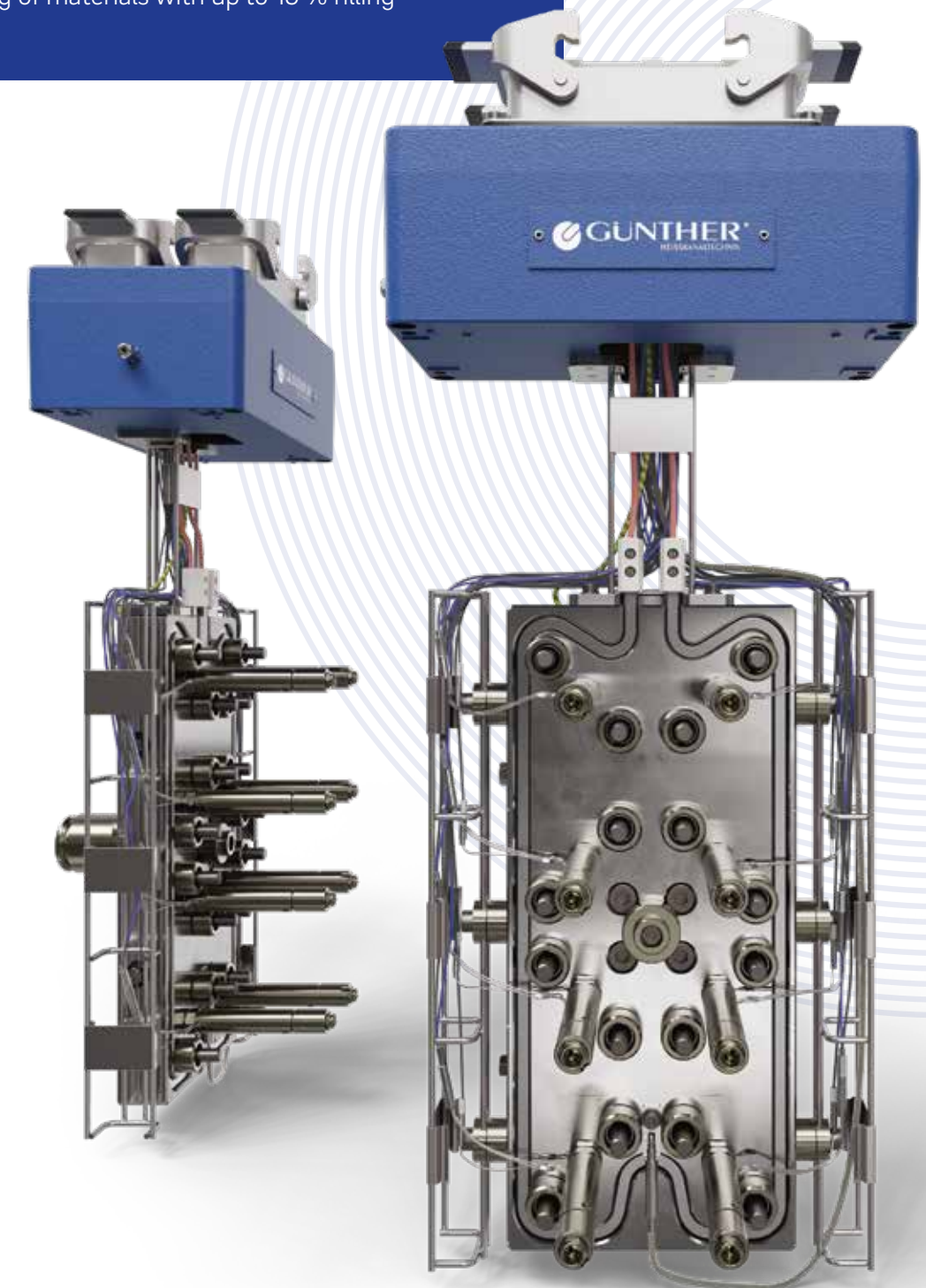
Basic2Connect system with nozzle type 6 8-drop H-Manifold
